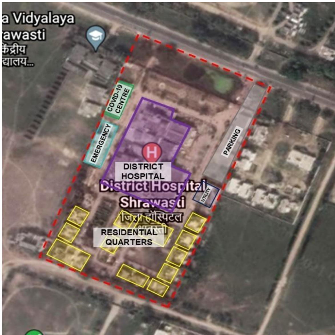
Site demarcation for District Hospital
